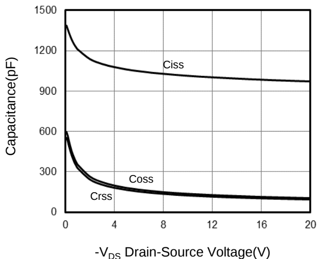
Figure 5. Capacitance
