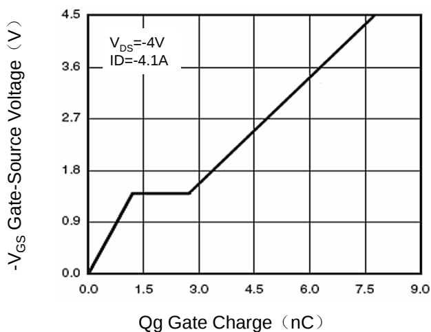
Figure 3. Gate Charge
